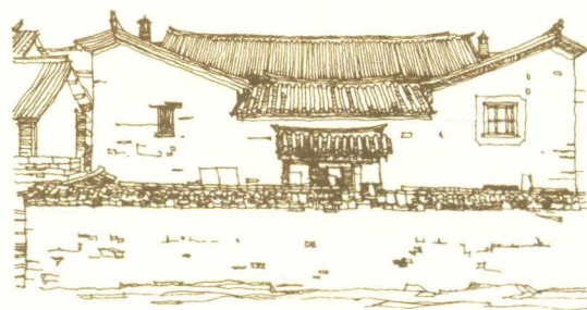
云南一颗印
