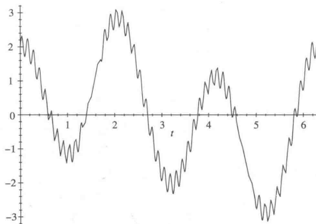
图1 f(t) = \sin(t) + 2 \cos(3t) + 0.3 \sin(50t)
