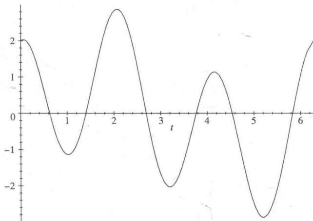
图2 f(t) = \sin(t) + 2 \cos(3t)
