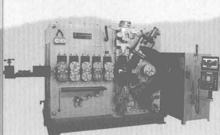
CK590, CK5120, CK5160, CK5180, CK5200 各型号六轴数控弹簧成形机 Wire Diameter(mm): \phi 3 \sim 20
