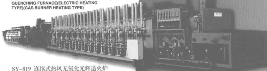
SY-819 连续式热风无氧化光輝退火炉 CONTINUOUS HOT BLAST NON-OXIDATION ANNEALING BRIGHT ANNEALING FURNACE
