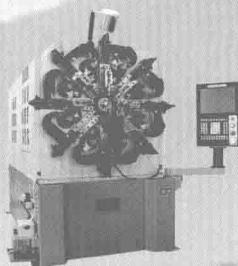
CNC642A 型数控万能弹簧转线成形机 Wire Diameter (mm): \phi 1.4 \sim 4.2
