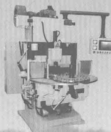
MK9 型新型双料盘数控磨簧机 Wire Diameter (mm): \phi 1 \sim 9 (MK3-MK6-MK9)
