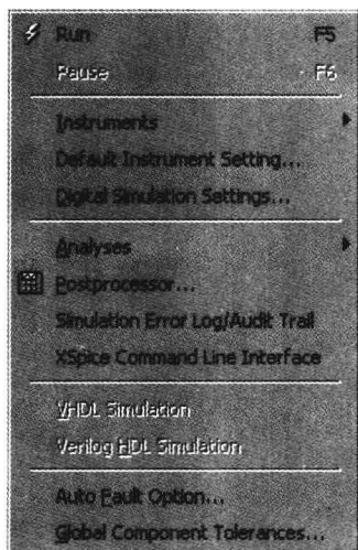
图 1-13 “Simulate”菜单
