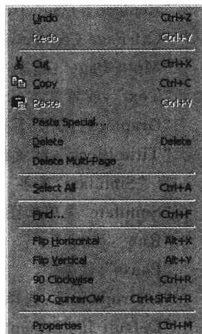
图 1-10 “Edit”菜单
