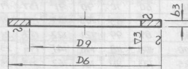
2-翼环
