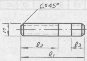
6-双头螺栓
