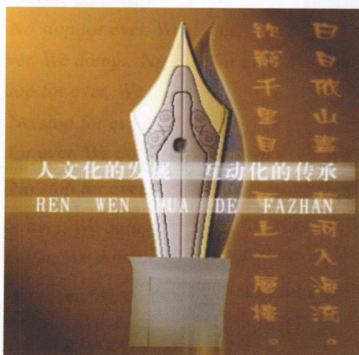
Xps3-05
