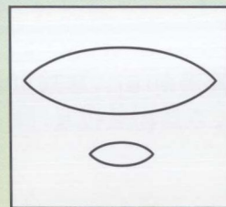
[au]
