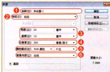
“新建”对话框
