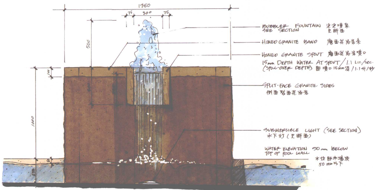
GRANITE FOUNTAIN BASIN ELEVATION
