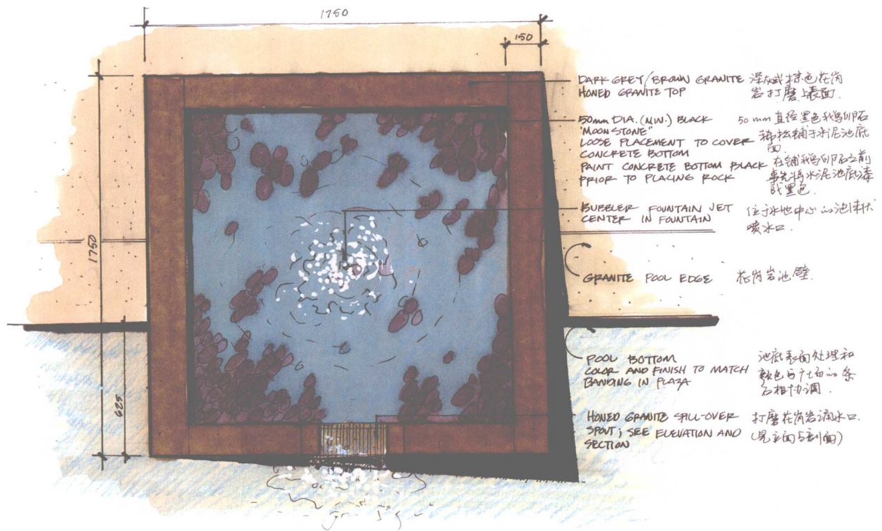
GRANITE FOUNTAIN BASIN PLAN VIEW
