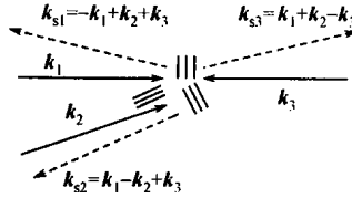
Fig. 1.1. Schematic diagram of phase-conjugate FWM.
