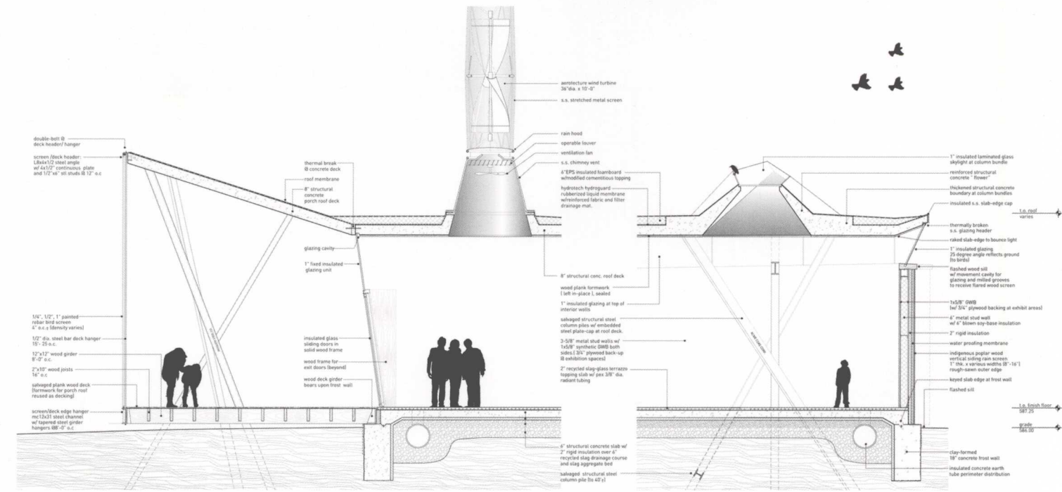
Sections showing construction detail and environmental systems in sustainable context 建筑细部和可持续环境系统剖面图
