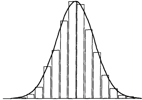
Figure I .1.2 Normal Distribution
