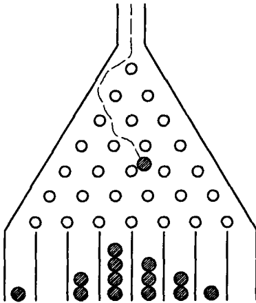
Figure I .1.1 Galton Board Experiment
