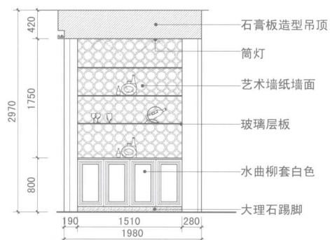
餐厅立面图 Elevation(Dining Room)
