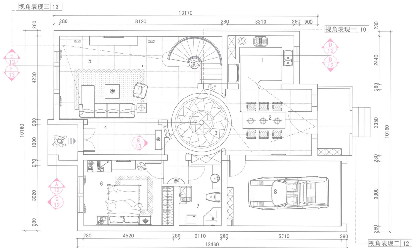
地面平面图/floor Plan
