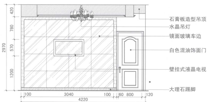
餐厅立面图 Elevation(Dining Room)
