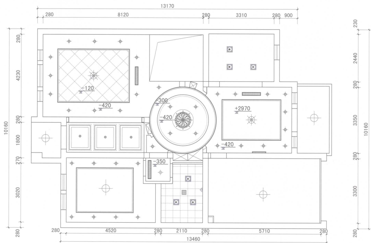
顶棚平面图/ceiling Plan
