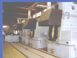
多用途热处理炉 采用国际先进技术制造的多用炉，用于销轴、滚子、套筒C-N共渗热处理 Multi-purpose furnace Multi-purpose furnace which made adopting international advanced technical used for pin, roller & bush carbon-nitriding heat treatment.
