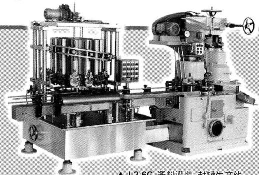
▲ L2-6C 酱料灌装-封罐生产线 VISCOUS LIQUID FILLING-SEAMING LINE
