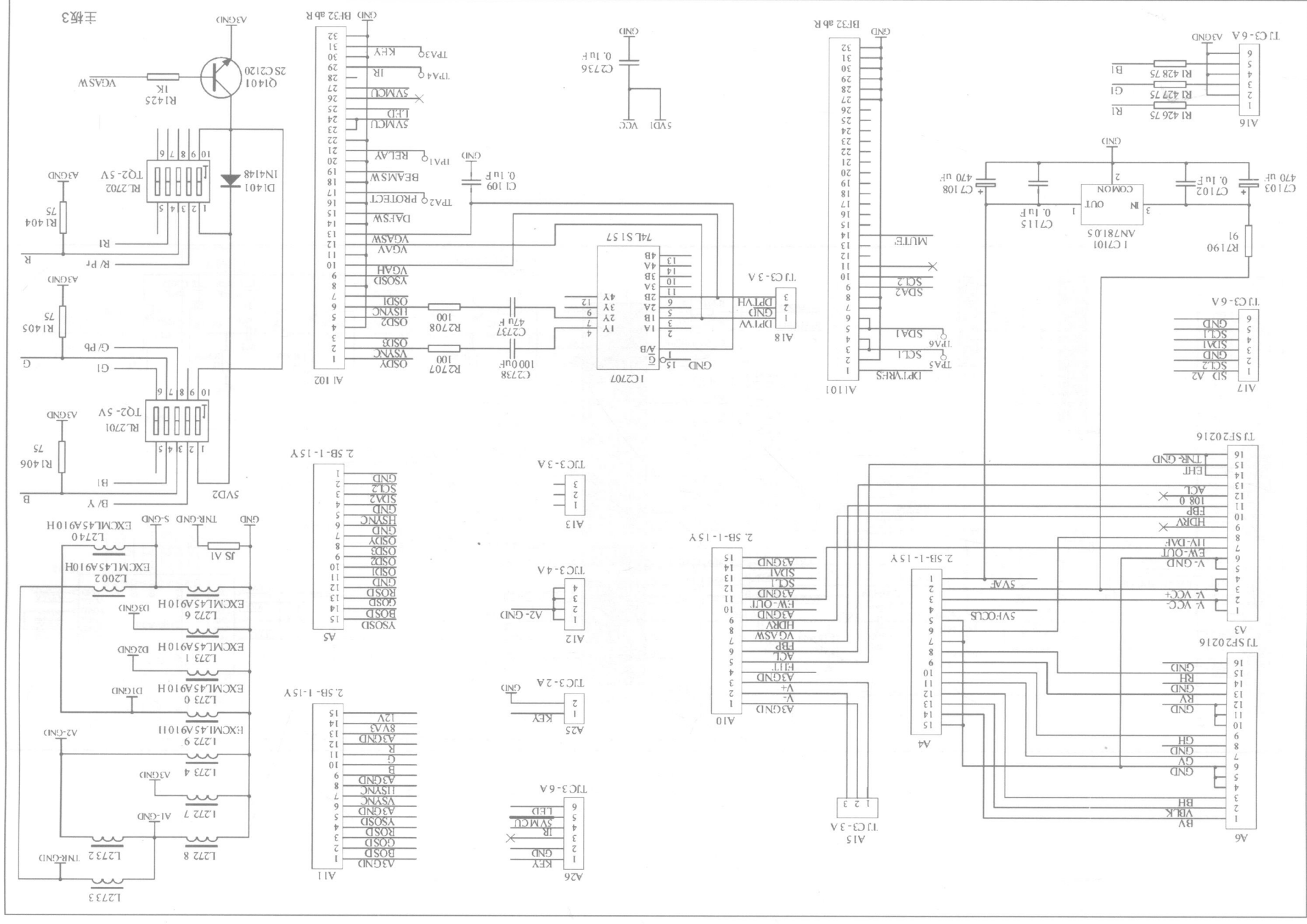
43PTV 机芯彩色电视机电路原理图(3/13)
