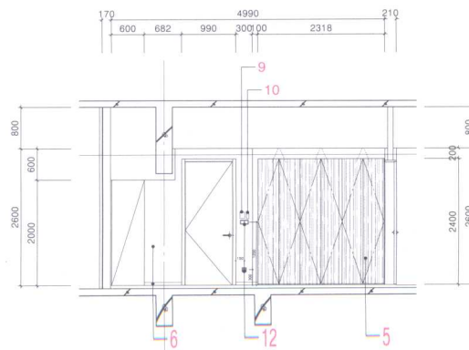
2层B型房立面图L
