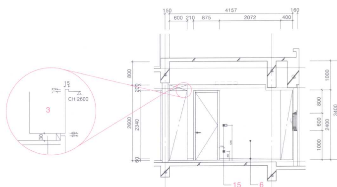
2层B型房立面图J
