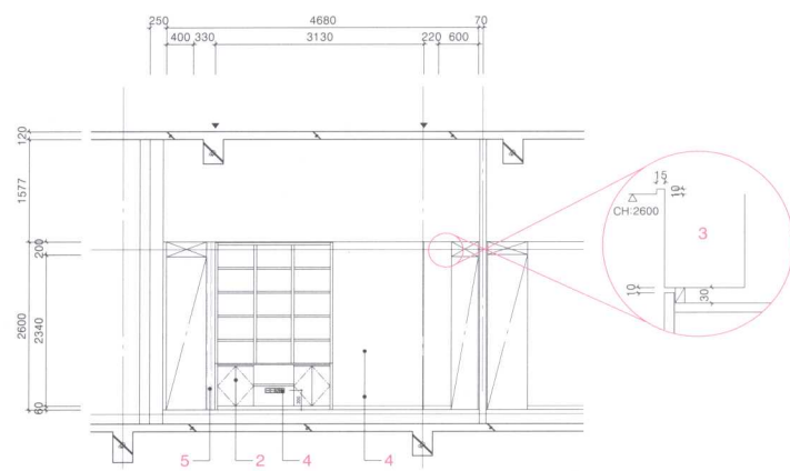
2层A型房立面图F
