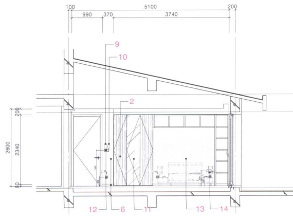
2层A型房立面图H
