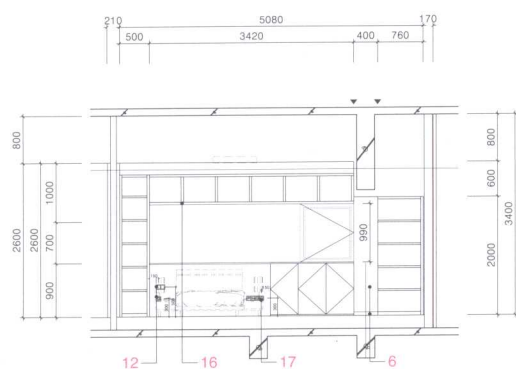
2层B型房立面图I
