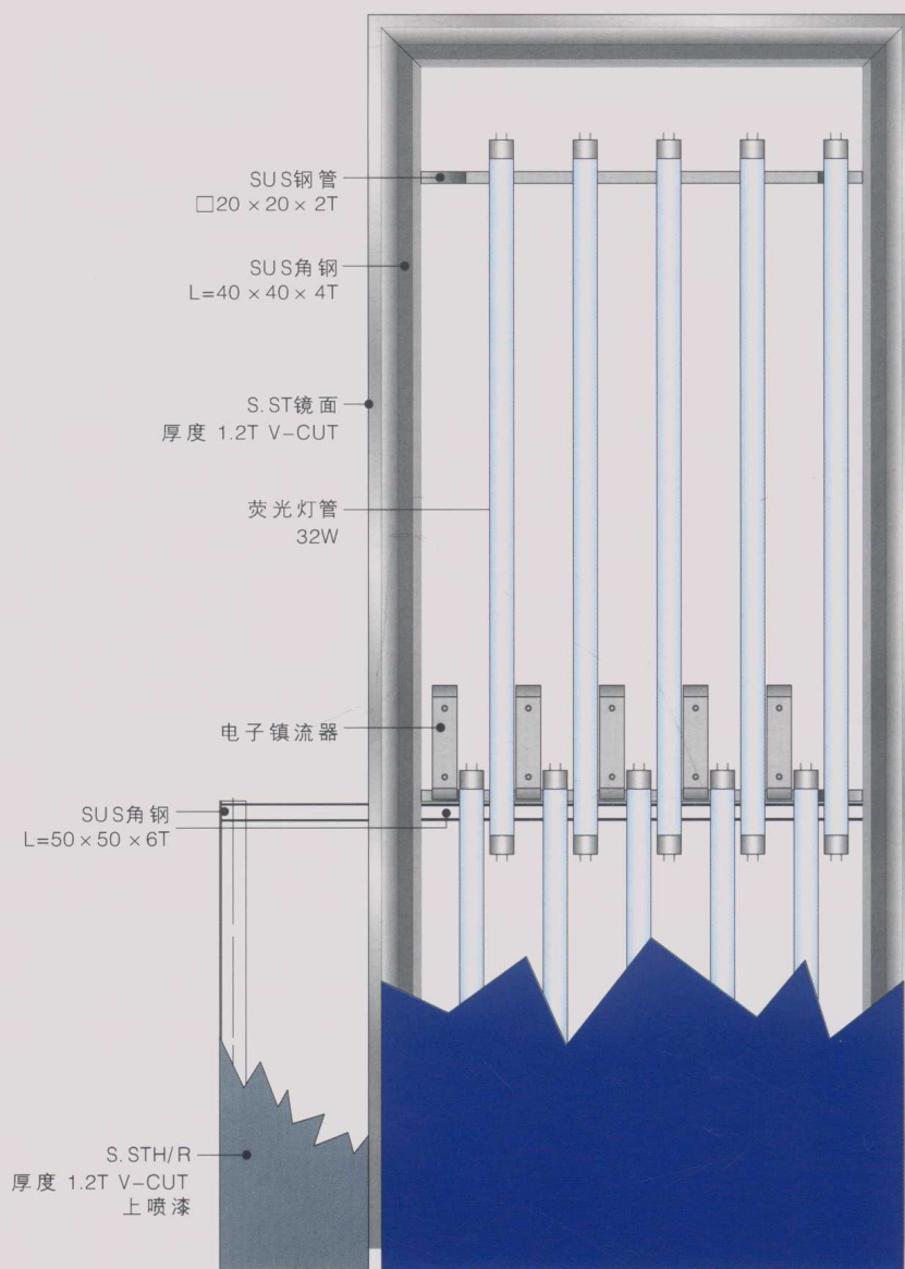
伸出式标识 Projecting sign
