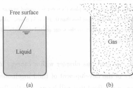
Fig. 1-1 (a) Liquid with a free surface and a definite volume; (b) Gas which expands freely with no free surface
