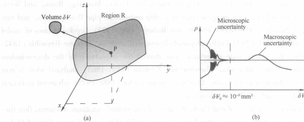
Fig. 1-2 The definition of continuum fluid density: (a) an elemental volume in a fluid region; (b) calculated density versus size of the elemental volume
